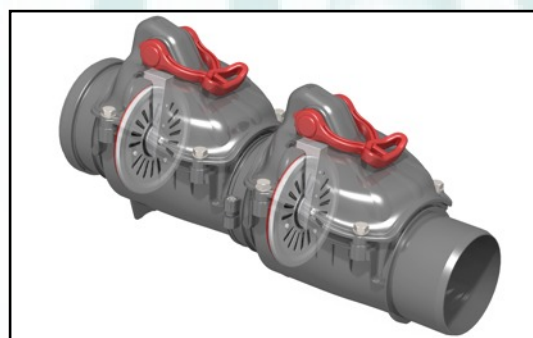
Double-flap backflow prevention valve
