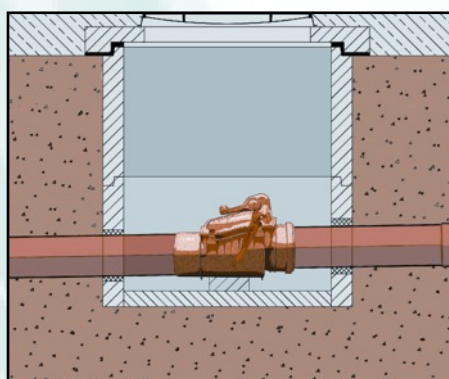
Installation in an access chamber.
